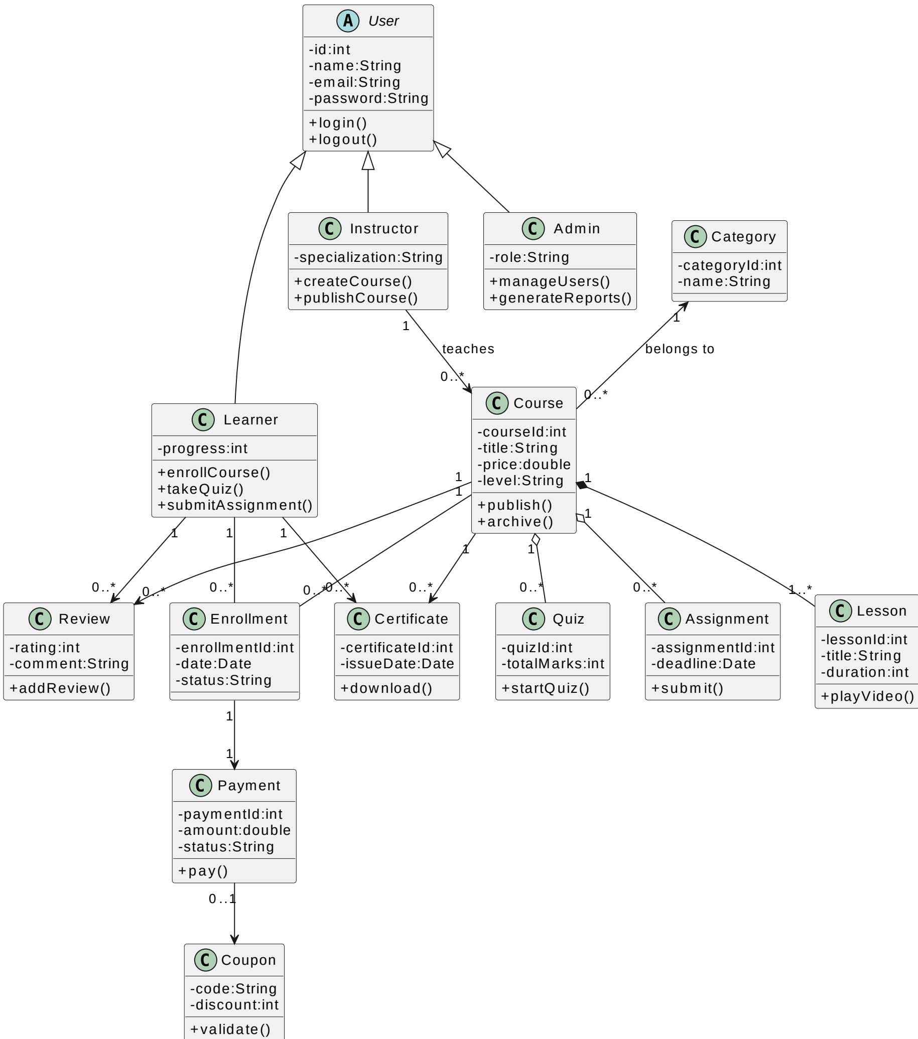
Online Course Learning System - Class Diagram
